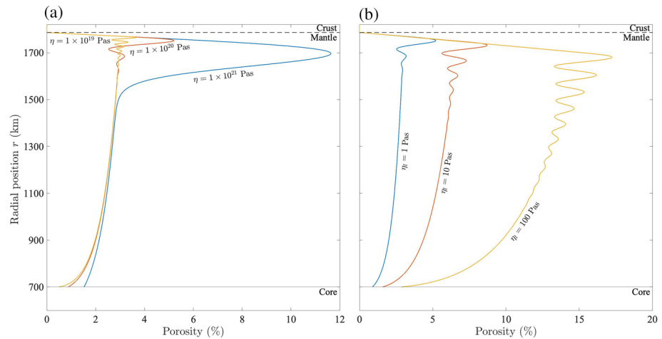
Figure 7. Porosity distribution for varying (a) shear viscosity and (b) melt viscosity. High shear viscosities cause thick decompacting boundary layers with high peak porosities. High melt viscosities cause high-melt-fractions throughout the mantle as melt can less easily segregate. High shear viscosity and low melt fractions increase the bulk viscosity, damping porosity oscillations.
