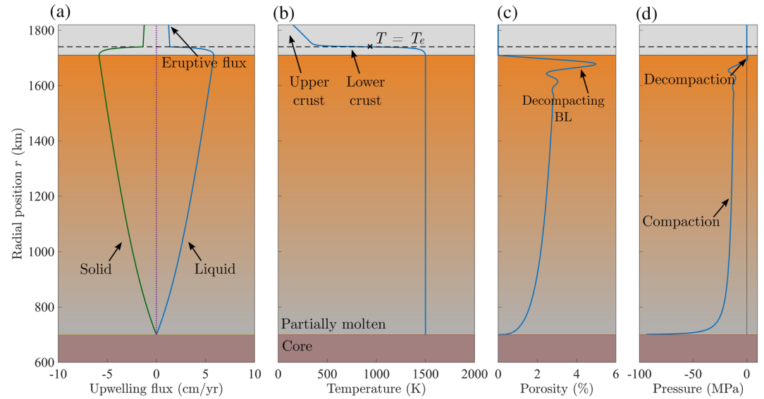
Figure 2. Example solution to the model with h = 7 \text{ Myr}^{-1} , T_e = 960 \text{ K} . (a) Upwelling magma is replaced by downwelling solid. (b) The lower crust ( T > T_e ) is heated by magmatic intrusions (emplacement), but the upper crust ( T < T_e ) is cold due to the downwelling cold surface material. (c) Melt fractions are low throughout the mantle but increase in a thin boundary layer on the order of 50 km thick. (d) Compaction occurs throughout most of mantle as the liquid is at low pressure, but beneath the crust P \simeq P_c = 0.8 \text{ MPa} , and downwelling solid is decompressed by liquid pressure. The elastic thickness is 80 km and the eruption rate is 1.1 cm/yr, with 99.5% of heat transport through the surface being volcanic. Parameter values can be found in Table 1.
