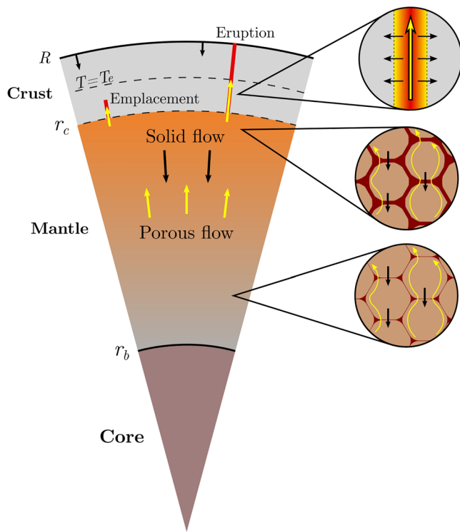
Figure 1. Schematic of the model for Io. Magma rises buoyantly through the mantle, while the solid moves downward. At the top of the mantle, magma enters the volcanic plumbing system. Some of this magma is emplaced (intruded) into the ductile lower crust; the rest rises to the surface and fuels volcanic eruptions. The core is excluded from the model.
