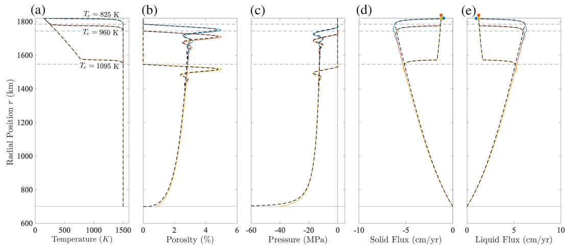
Figure 4. The effect of elastic limit temperature T_e on (a) temperature profile, (b) porosity distribution, (c) compaction pressure, and (d) solid and (e) liquid fluxes. Solid lines are full solutions to the model, and heavy dashed lines are the approximate solutions. As the elastic limit temperature T_e is increased, crustal thickness increases and a larger proportion of the upper crust is cold, resulting in larger elastic thicknesses. h = 7 \text{ Myr}^{-1} in these solutions.
