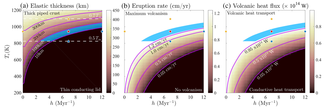
Figure 5. Model predictions of (a) elastic thickness, (b) eruption rate, and (c) volcanic heat flux in the parameter space of emplacement constant h and elastic limit temperature T_e . The dashed lines on panel (a) mark homologous temperatures 0.5T_m and 0.7T_m , an estimated range for the transition from brittle to ductile behavior. The blue region covers the parameter space for potential elastic thicknesses (10–100 km). The central red star marks the solution displayed in Figure 2, and other stars mark the solutions in Figures 3 and 4.
