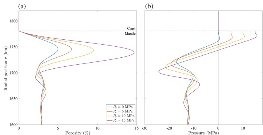
Figure 6. (a) Porosity and (b) compaction pressure in the decompacting boundary layer beneath the crust for different values of critical compaction pressure P_c . High values of P_c cause the material downwelling from the crust to decompact rapidly, leading to the accumulation of large amounts of melt. Note the different radial scale from other figures.
