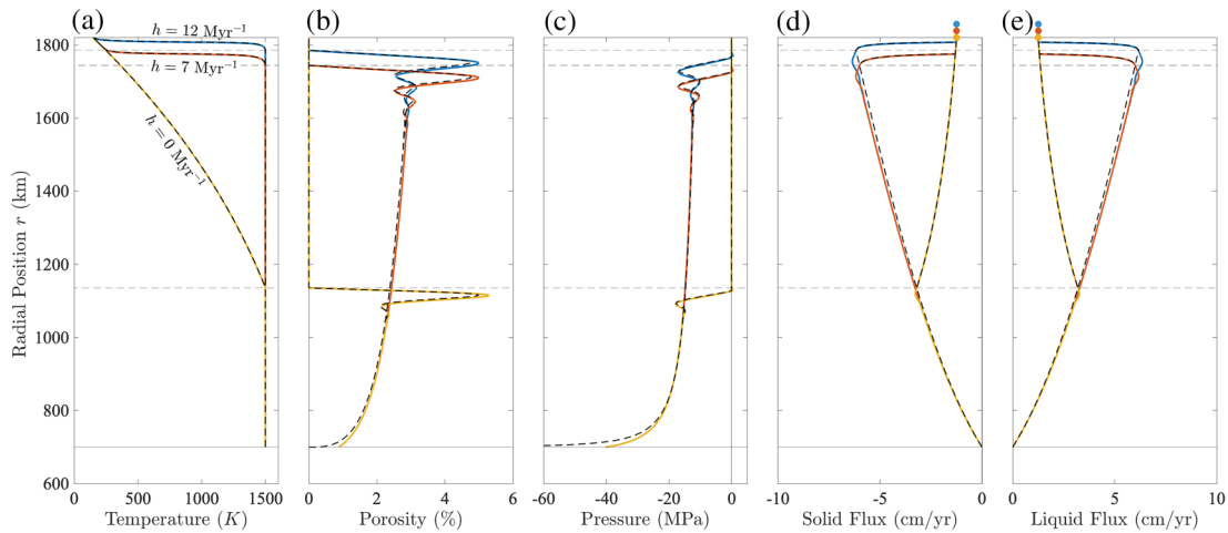
Figure 3. The effect of emplacement rate h on (a) temperature profile, (b) porosity distribution, (c) compaction pressure, and (d) solid and (e) liquid fluxes. Solid lines are full solutions to the model, and heavy dashed lines are the approximate solutions. Thin dashed lines mark the crust-mantle boundaries. Dots on panels (d) and (e) show the surface erupted fluxes. When there is no magmatic emplacement ( h = 0 ), the crust grows to be over 600 km thick due to the rapid downwelling of the cold surface temperature. As emplacement rate is increased, the heating that this provides to the crust can increasingly balance the cold downwelling surface temperature, resulting in smaller crustal thicknesses. T_e = 960 \text{ K} in these solutions. Liquid flux is the sum of the segregation flux q and plumbing system flux q_p . Parameter values can be found in Table 1.
